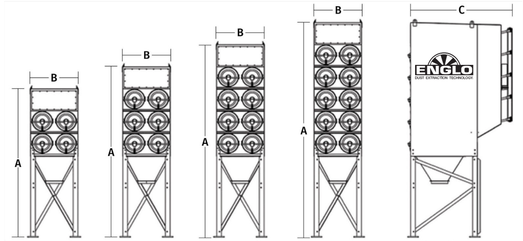
ENGLO 2 Series ENGLO 3 Series ENGLO 4 Series ENGLO 5 Series Side View
